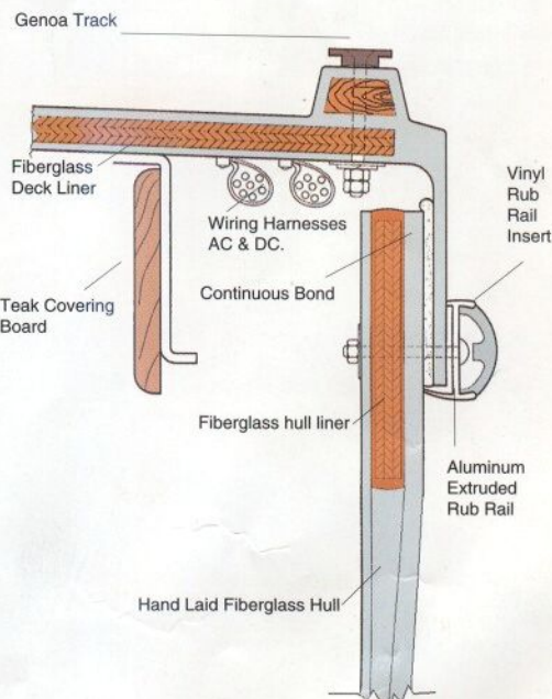
TYPICAL HULL AND DECK SECTION
